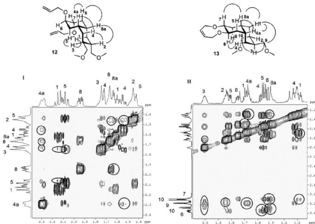
Figure 2. Sections of the NOESY spectra of 10b (left) and 11b (right) in \text{CDCl}_3 and structures of their corresponding conformers 12 and 13 with significant NOE contacts.
