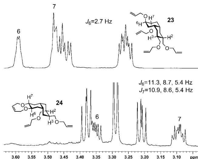
Figure 4. Parts of the ^1\text{H} NMR spectra of compounds 19 (top) and 21 (bottom) showing the presence of the conformers 23 and 24 . The diagnostic coupling constants of H-C6,7 are highlighted.
