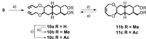
Scheme 3. RCM reaction of the bis(allyl ethers) 10 to the eight-membered ring products 11 : a) i) allyl bromide, NaH, DMF, 16 h; ii) TBAF, THF, 2 h 40^\circ\text{C} , 93% 10a in two steps; b) MeI, NaH, DMF, 16 h, 93% 10b ; c) \text{Ac}_2\text{O} , Py, DMAP, 6 h, 88% 10c ; d) 10b \rightarrow 11b , Grubbs I catalyst, toluene, 140^\circ\text{C} , sealed tube, 30 min, 98%; 10c \rightarrow 11c , Grubbs I catalyst, \text{ClCH}_2\text{CH}_2\text{Cl} , 85^\circ\text{C} , 1 h, 76%; e) 11c \rightarrow 10c , Grubbs I catalyst, \text{CH}_2\text{Cl}_2 , room temp., 4 bar ethylene, 22 h, 62%.
