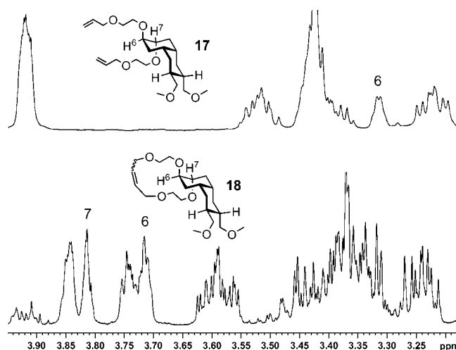
Figure 3. Parts of the ^1\text{H} NMR spectra of compounds 15 (bottom) and 16 (top) showing the presence of the conformers 17 and 18 . The diagnostic signals of H-C6,7 are highlighted.
