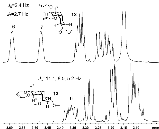
Figure 1. Parts of the ^1\text{H} NMR spectra of compounds 10b (top) and 11b (bottom) showing the presence of the conformers 12 and 13 . The diagnostic coupling constants of H-C6,7 are highlighted.
