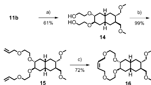
Scheme 4. Synthesis and RCM reaction of the bis(allyl ether) 15 to the 14-membered-ring product 16 : a) \text{O}_3 , \text{NaBH}_4 , \text{CH}_2\text{Cl}_2/\text{MeOH} (1:1), 16 h; b) allyl bromide, \text{NaH} , DMF, 16 h; c) Grubbs I, toluene, 140^\circ\text{C} , sealed tube, 30 min.
