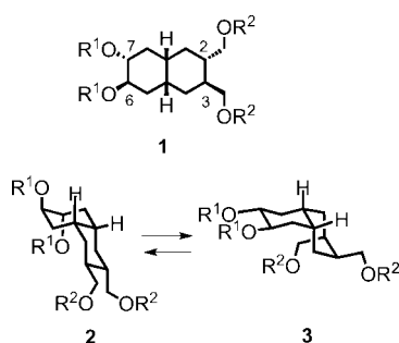
Scheme 1. Decalin 1 and the double-ring flip interconverting conformers 2 and 3 .
