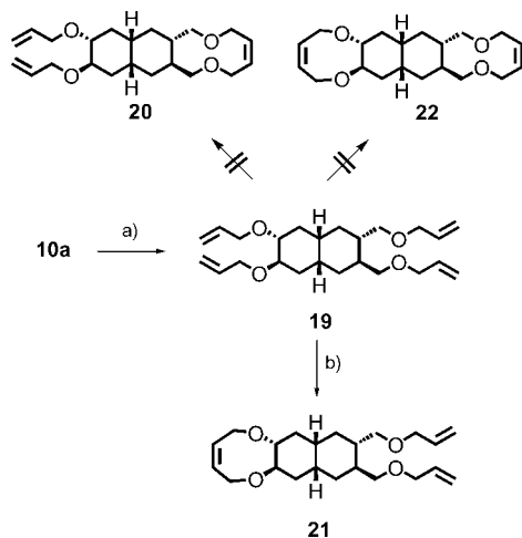
Scheme 5. Synthesis and RCM reaction of 19 leading to 21 : a) allyl bromide, NaH, DMF, 16 h, 61%; b) Grubbs I catalyst, toluene, 140 °C, sealed tube, 30 min, 45%.
